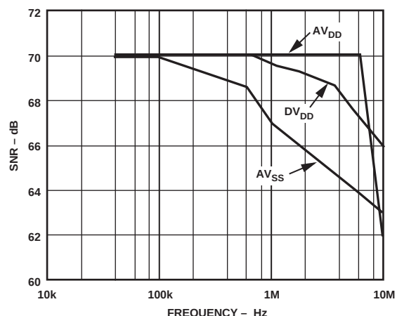
Figure 30. SNR vs. Supply Noise Frequency ( f_{IN} = 1 \text{ MHz} )
