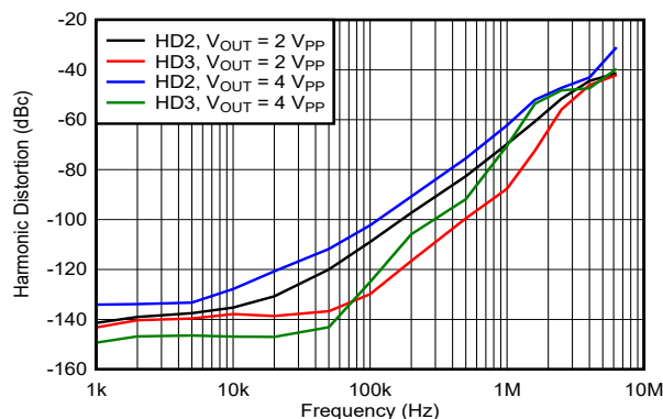
Distortion Performance in G = 1 V/V
