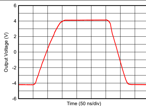
Figure 7-12. Large-Signal Transient Response
