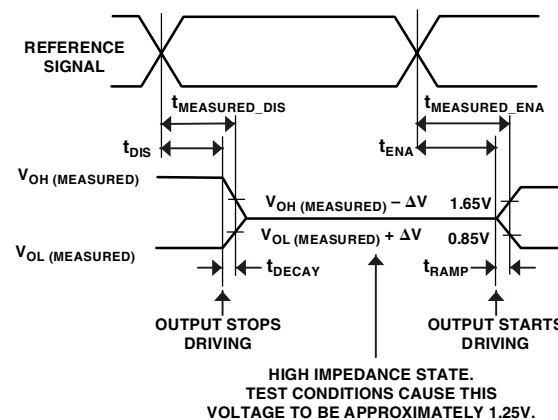
Figure 35. Output Enable/Disable
