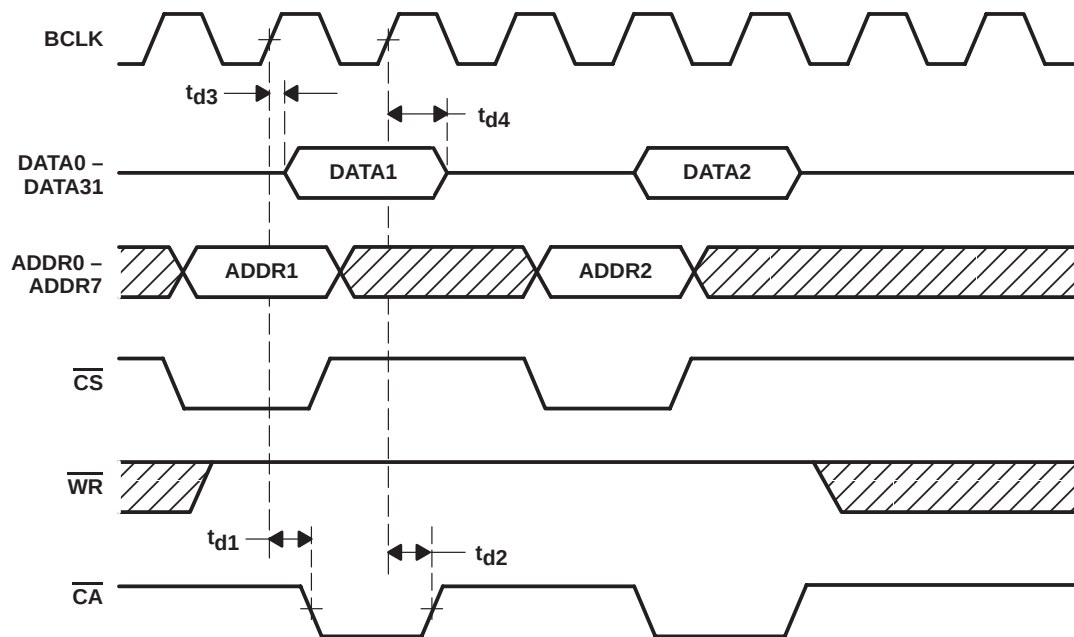
Figure 6-5. Host-Interface Quick Read-Cycle Waveforms ( \text{ADDR0} - \text{ADDR7} \geq 30\text{h} )
