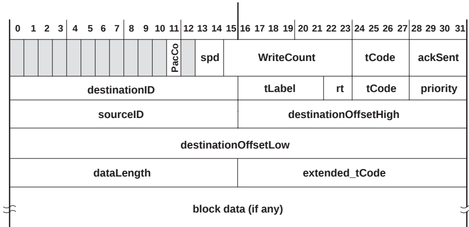
Figure 4–4. Block-Receive Format
