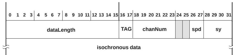
Figure 4–5. Isochronous-Transmit Format
