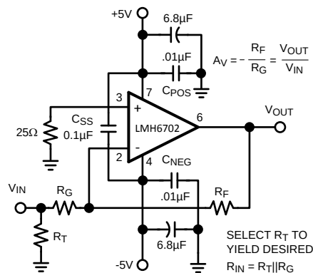
Figure 22. Recommended Inverting Gain Circuit
