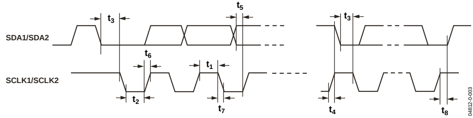
Figure 3. I²C Timing
