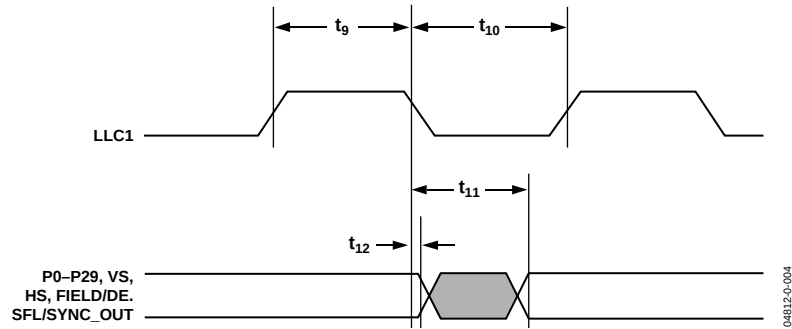
Figure 4. Pixel Port and Control Output Timing (SD Core)
