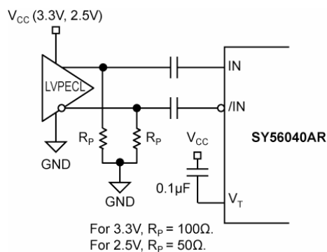
Figure 4d. LVPECL Interface (AC-Coupled)
