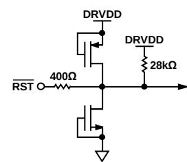
Figure 41. Equivalent \overline{RST} Input Circuit
