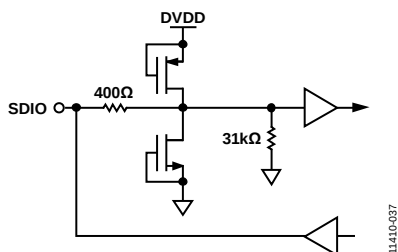
Figure 37. Equivalent SDIO Circuit
