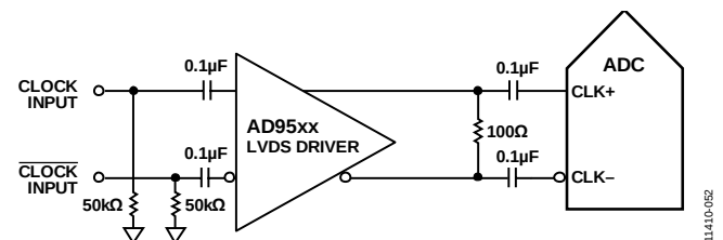
Figure 52. Differential LVDS Sample Clock (Up to 625 MHz)
