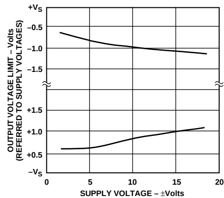
Figure 18. Output Voltage Limit vs. Supply Voltage
