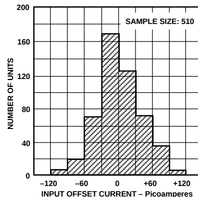
Figure 3. Typical Distribution of Input Offset Current
