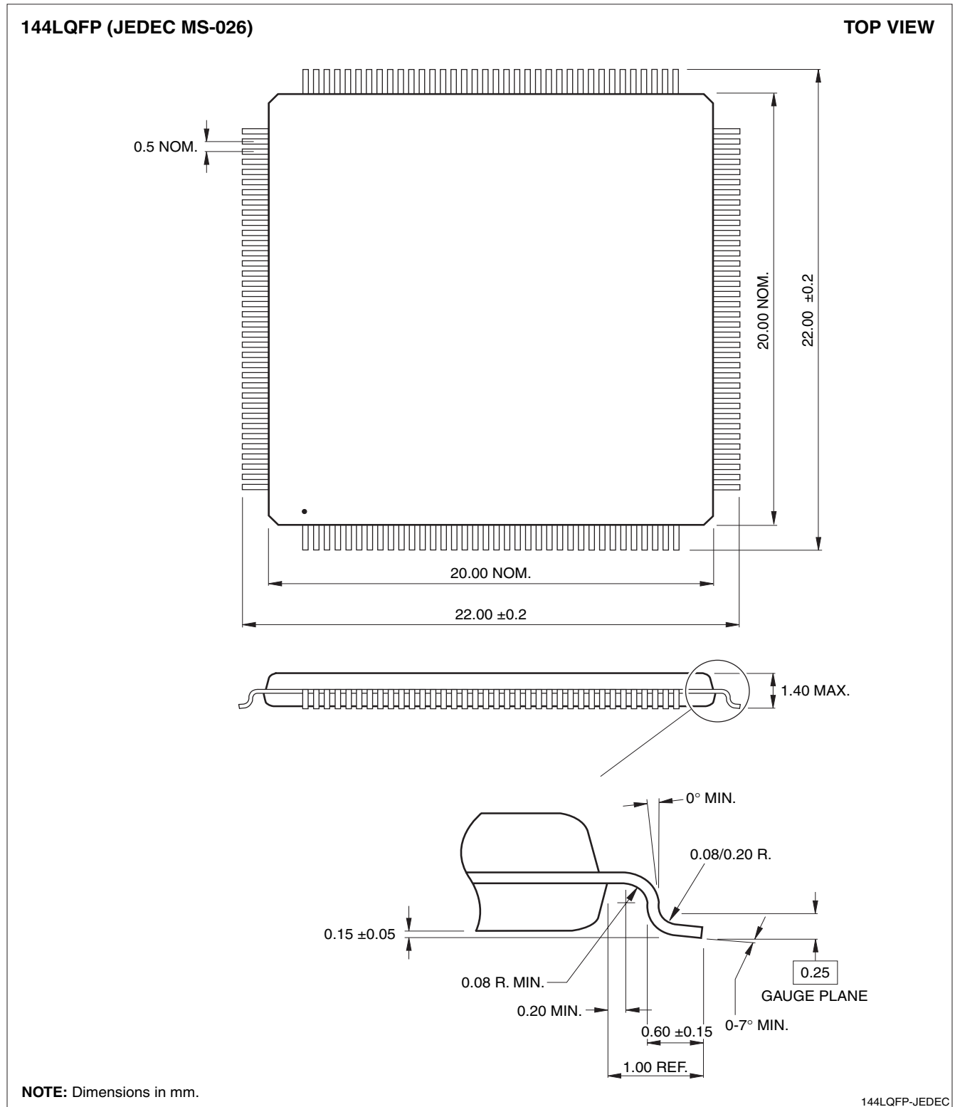
Figure 28. 144-pin LQFP
