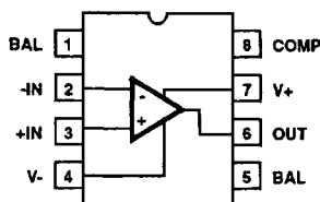
HA-2600/883, HA-2602/883 (CERDIP) TOP VIEW
