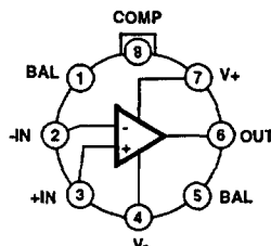
HA-2600/883, HA-2602/883 (METAL CAN) TOP VIEW
