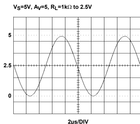
FIGURE 24. OUTPUT SWING
