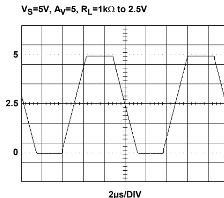
FIGURE 22. OUTPUT SWING
