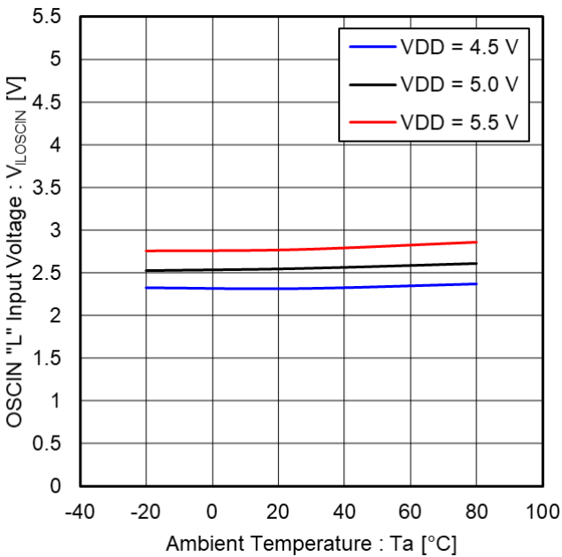
Figure 8. OSCIN "L" Input Voltage vs Ambient Temperature
