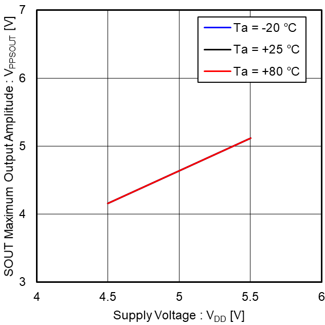
Figure 22. SOUT Maximum Output Amplitude vs Supply Voltage
