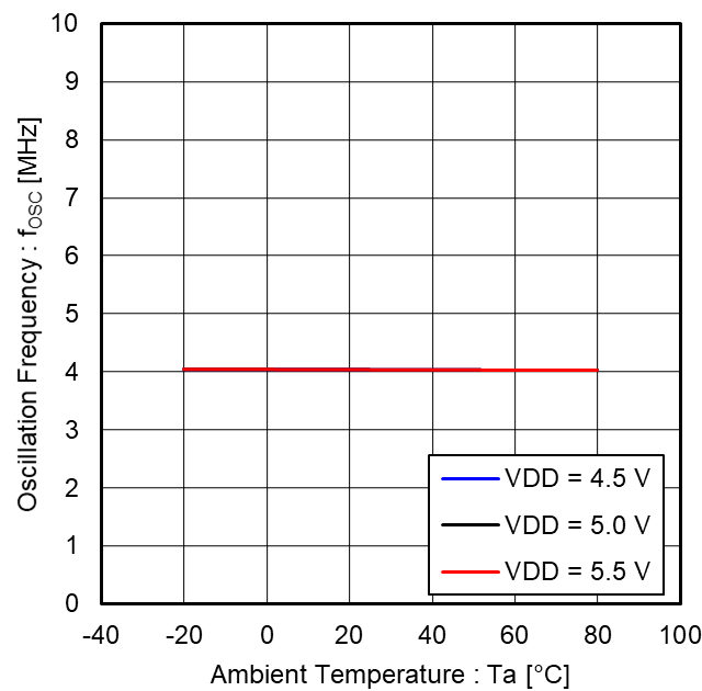
Figure 2. Oscillation Frequency vs Ambient Temperature
