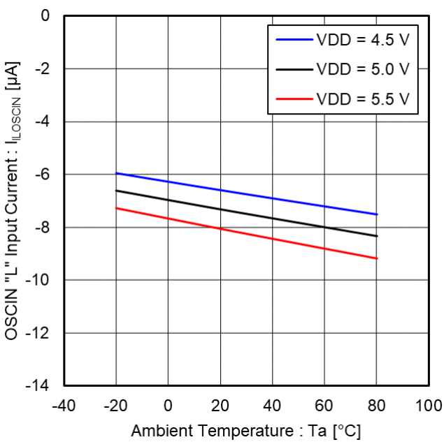
Figure 6. OSCIN "L" Input Current vs Ambient Temperature
