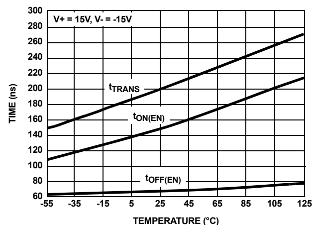
FIGURE 15. t_{\text{ON}}/t_{\text{OFF}} vs TEMPERATURE
