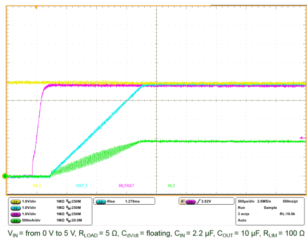
Figure 22. Startup via input voltage (5 \Omega load)
