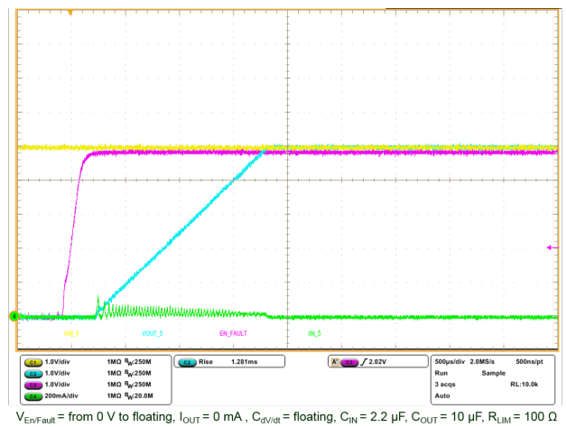
Figure 21. Startup via En/Fault pin (No load)
