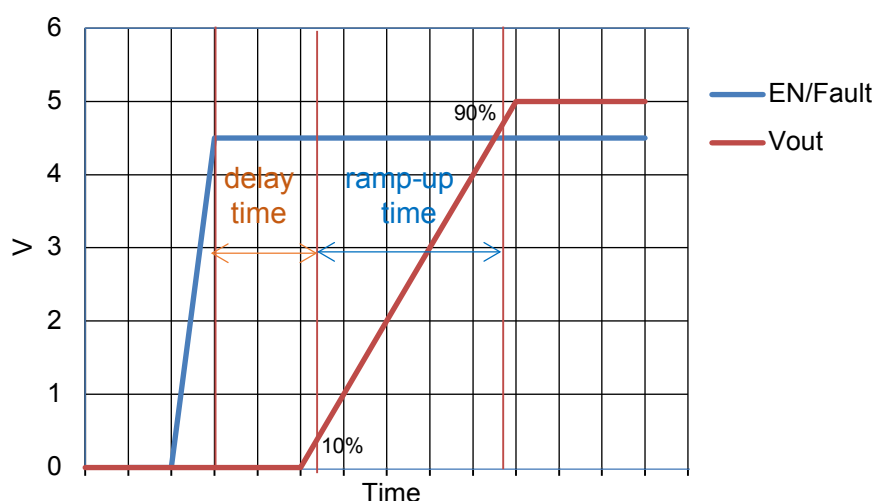
Figure 4. Delay time and V_{OUT} ramp-up time
