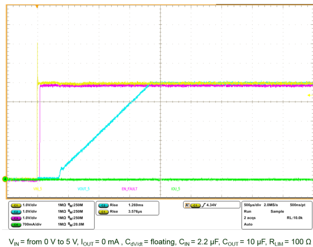
Figure 20. Startup via input voltage (No load)
