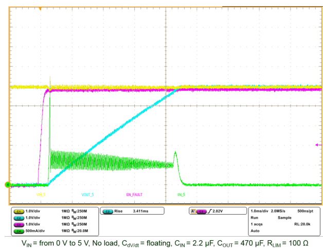
Figure 23. Startup via En/Fault ( C_{OUT} = 470 \mu F )
