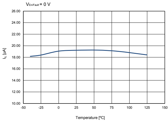
Figure 18. En/Fault pin current vs. temperature (En/Fault to GND)
