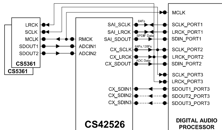
Figure 18. OLM Configuration #3
