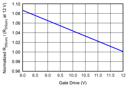
Figure 6-1. Normalized R_{DS(on)} vs Gate Drive
