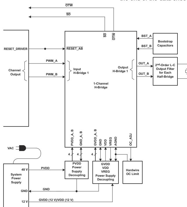
DRV2901 Functional Block Diagram
