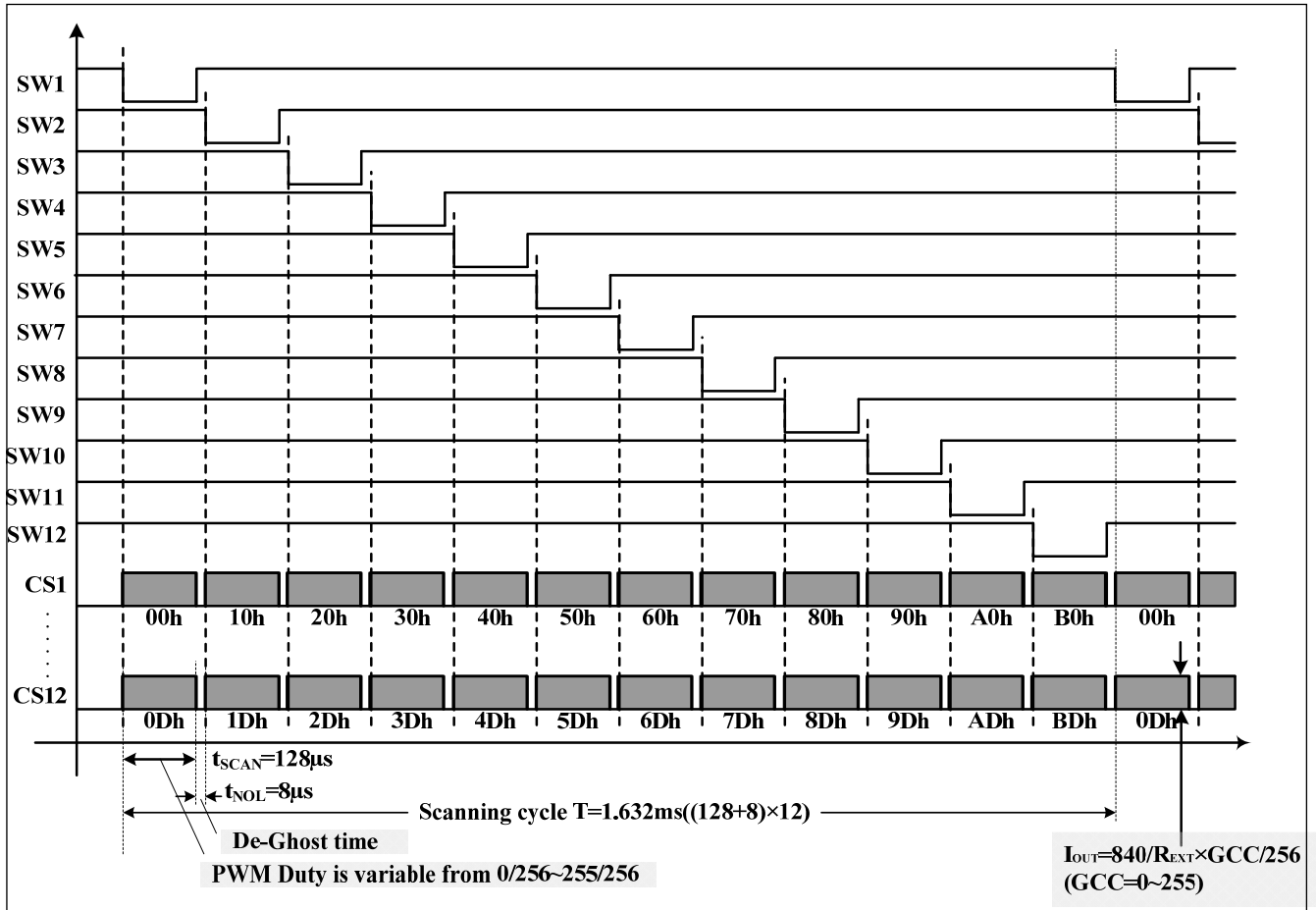
Figure 12 Scanning Timing
