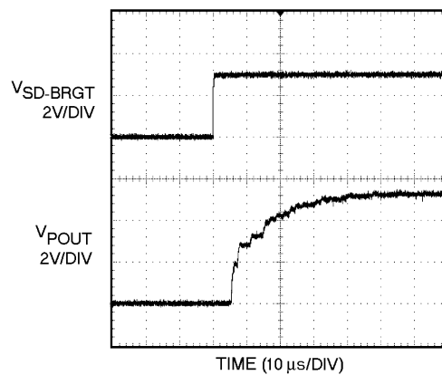
Startup Response
