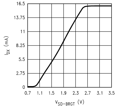
LED Current vs. SD-BRGT Voltage
