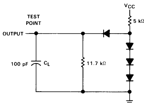
FIGURE 1. TEST CIRCUIT
