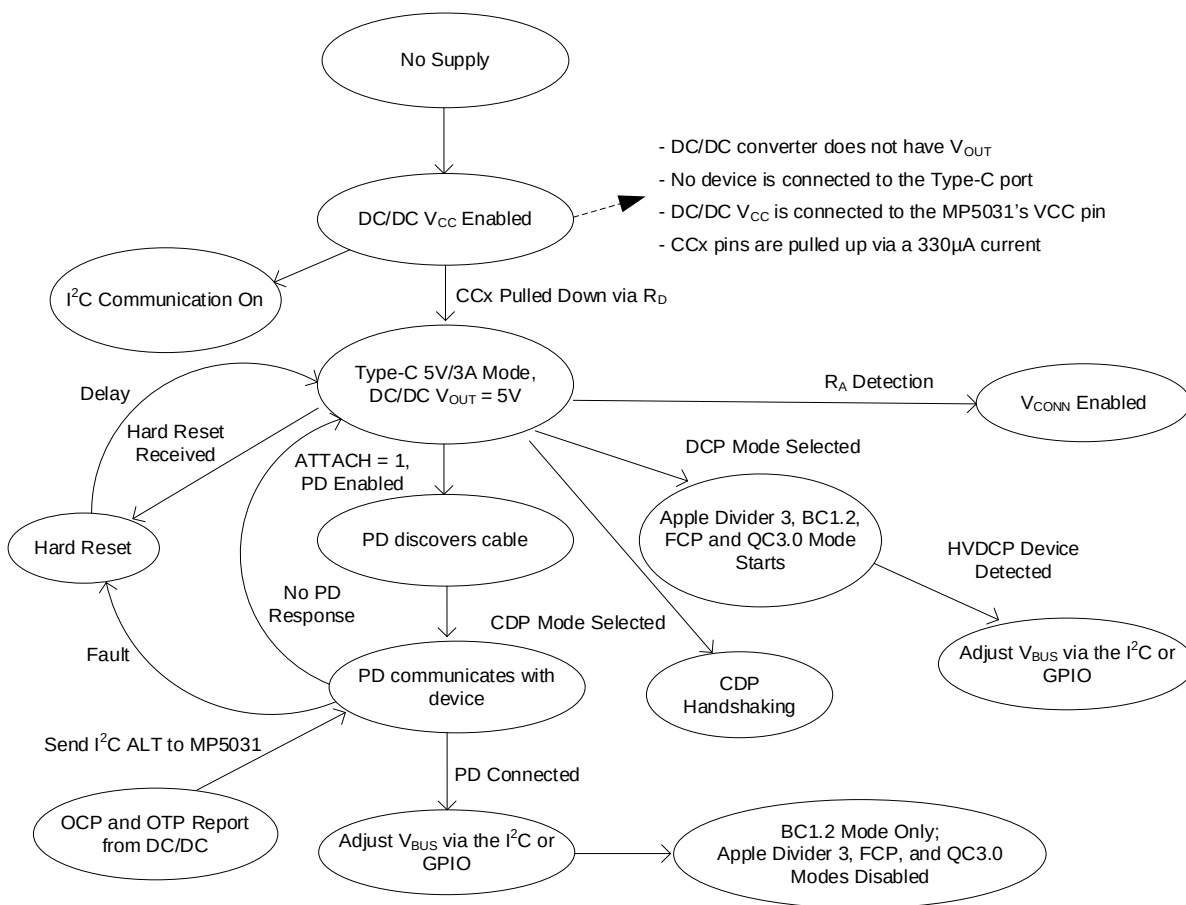
Figure 10: State Machine Diagram
