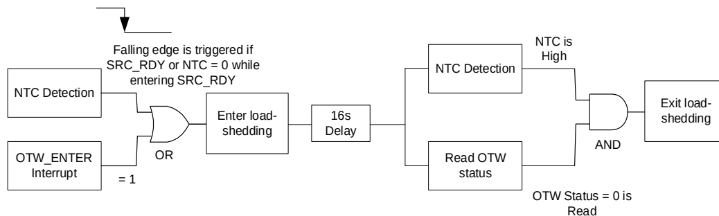
Figure 14: Load-Shedding Logic (6)
