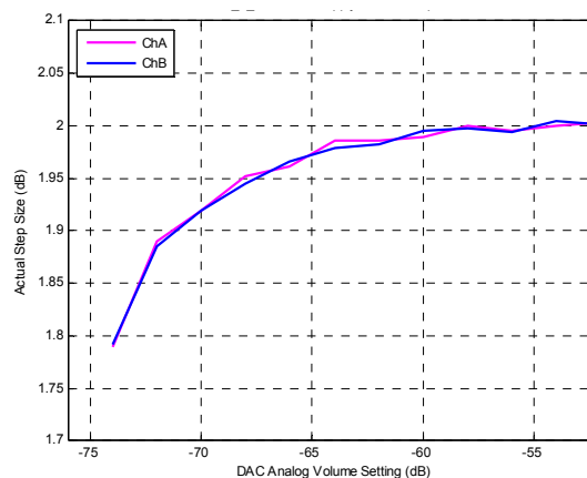
Figure 65. LINEOUTx DNL (-76 to -52 dB)
