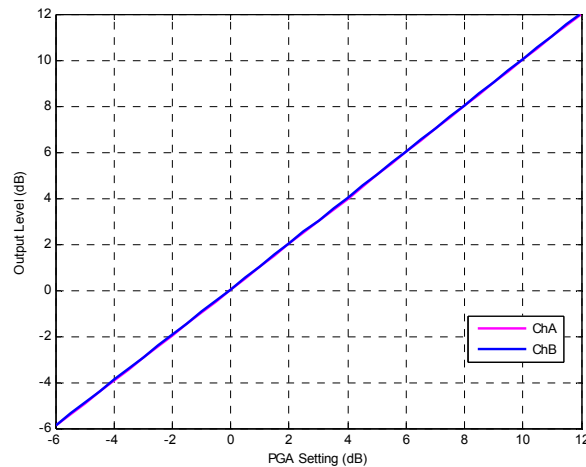
Figure 43. PGA INL
