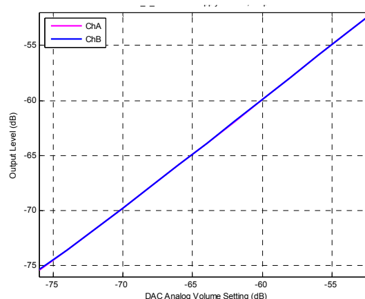
Figure 67. LINEOUTx INL (-76 to -52 dB)
