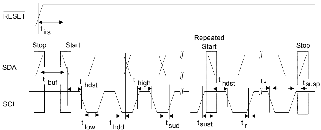
Figure 14. I²C Control Port Timing
