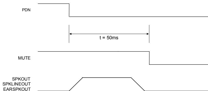
Figure 40. Fast Start Pop
