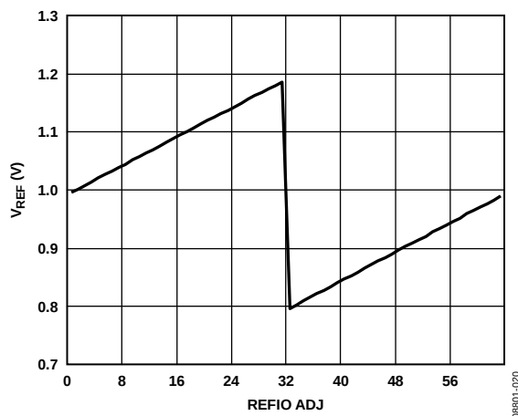
Figure 54. Typical V_{REFIO} Voltage vs. REFIO_ADJ Value
