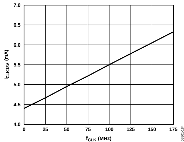
Figure 99. I_{CLKVDD18} vs. f_{CLK}
