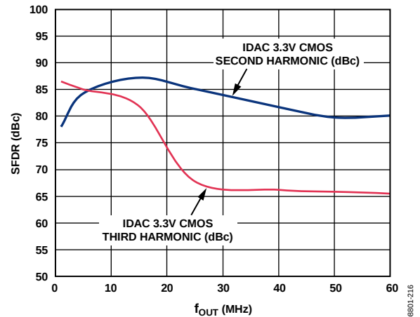
Figure 19. AD9961, Second and Third Harmonic Distortion vs. f_{OUT} , f_{DAC} = 125 MHz, 1×, Digital Scale = 0 dBFS, TXVDD = 3.3 V
