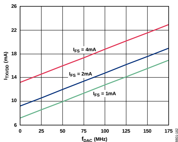
Figure 97. I_{TXVDD} vs. f_{DAC} FSC = 1\text{ mA}, 2\text{ mA}, 4\text{ mA} , TXVDD = 3.3\text{ V}
