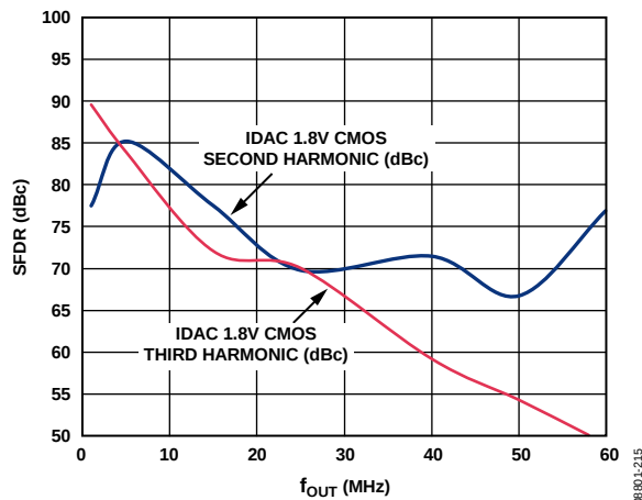
Figure 18. AD9961, Second and Third Harmonic Distortion vs. f_{OUT} , f_{DAC} = 125 MHz, 1×, Digital Scale = 0 dBFS, TXVDD = 1.8 V
