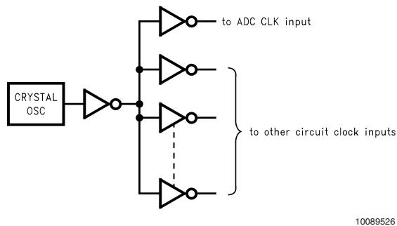
FIGURE 4. Isolating the ADC Clock from Digital Circuitry
