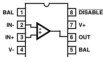
HA-5020 (PDIP, SOIC) TOP VIEW
