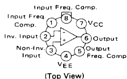
G SUFFIX METAL PACKAGE CASE 601
