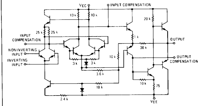
FIGURE 1 - EQUIVALENT CIRCUIT SCHEMATIC
