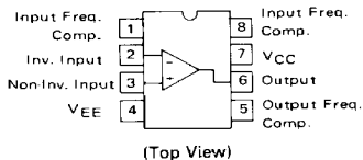
U SUFFIX CERAMIC PACKAGE CASE 693
