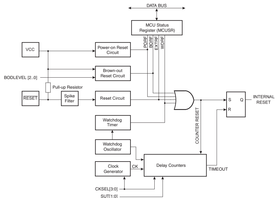
Figure 9-1. Reset Logic
