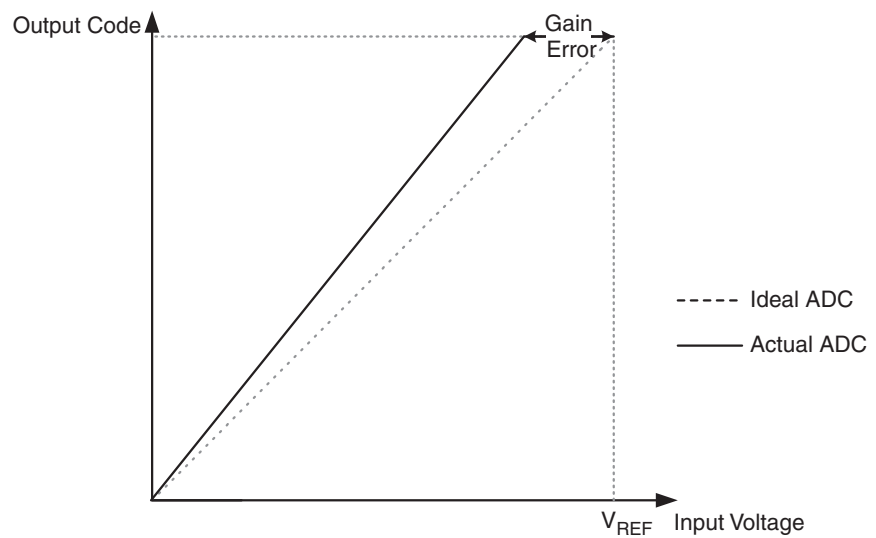
Figure 21-11. Gain Error
