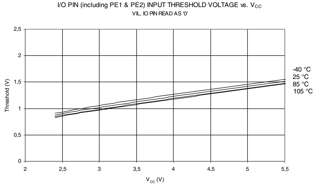
Figure 27-20. I/O Pin Input Threshold Voltage vs. V_{CC} ( V_{IL} , I/O Pin Read As '0')
