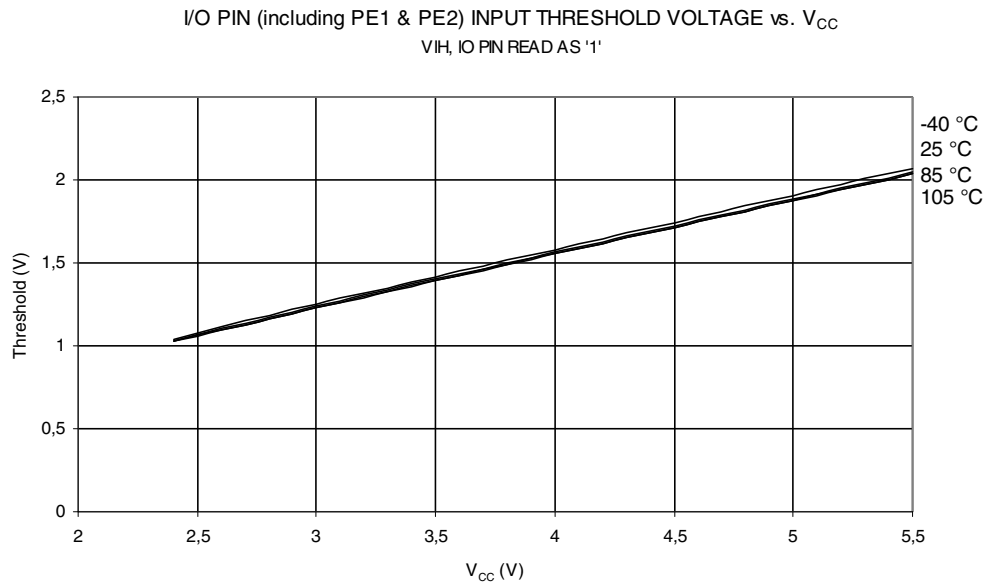
Figure 27-19. I/O Pin Input Threshold Voltage vs. V_{CC} ( V_{IH} , I/O Pin Read As '1')
