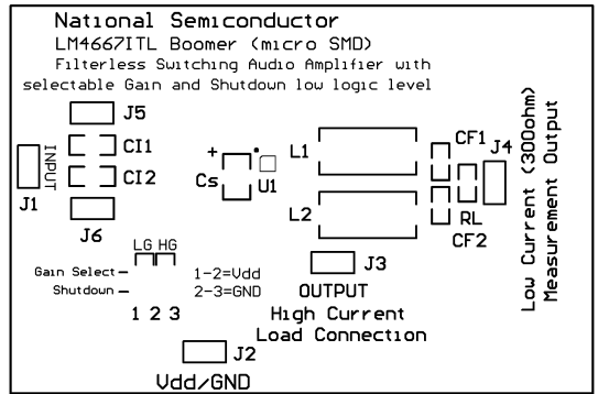
Silk Screen
