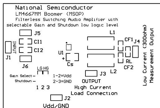
Silk Screen
