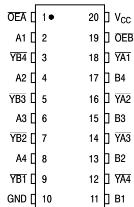
PIN ASSIGNMENT
