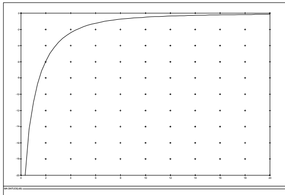
Figure 66 ADC Highpass Filter Response
