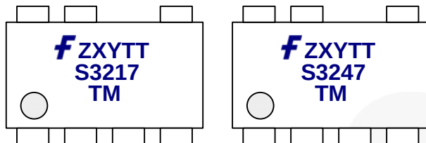
Figure 3. Top Mark
