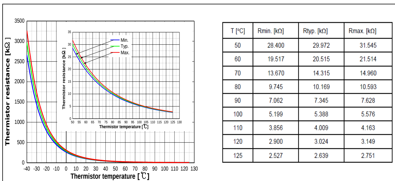
Figure 6 Thermistor resistance – temperature curve and table
