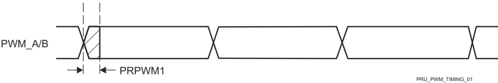
Figure 7-99. PRU_ICSSG PWM Timing
