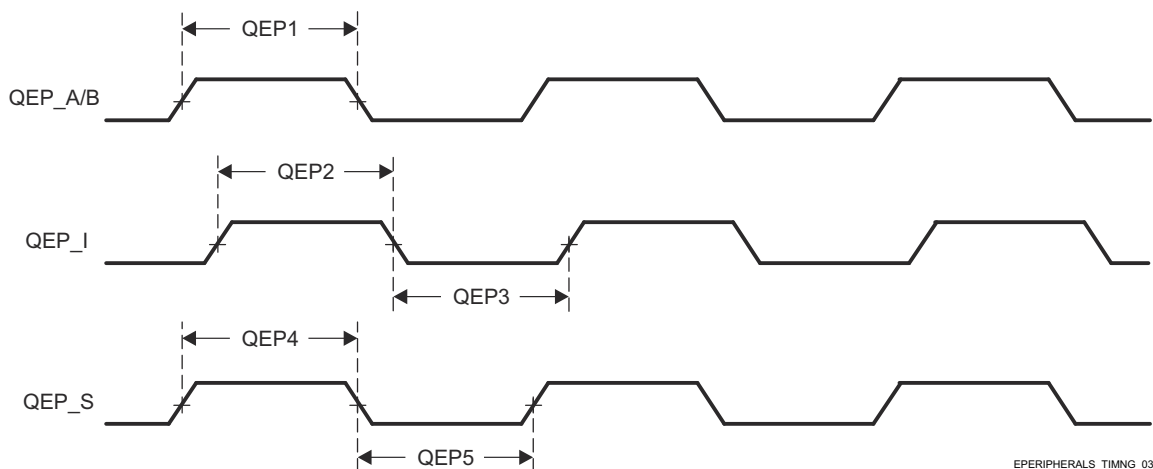
Figure 7-35. EQEP Timing Requirements
