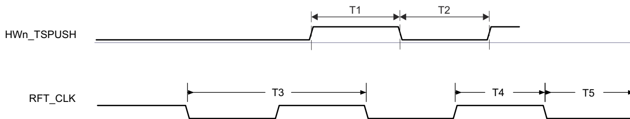
Figure 7-77. CPTS Timing Requirements
