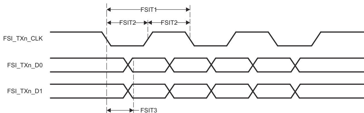
Figure 7-37. FSI Switching Characteristics - FSI Mode
