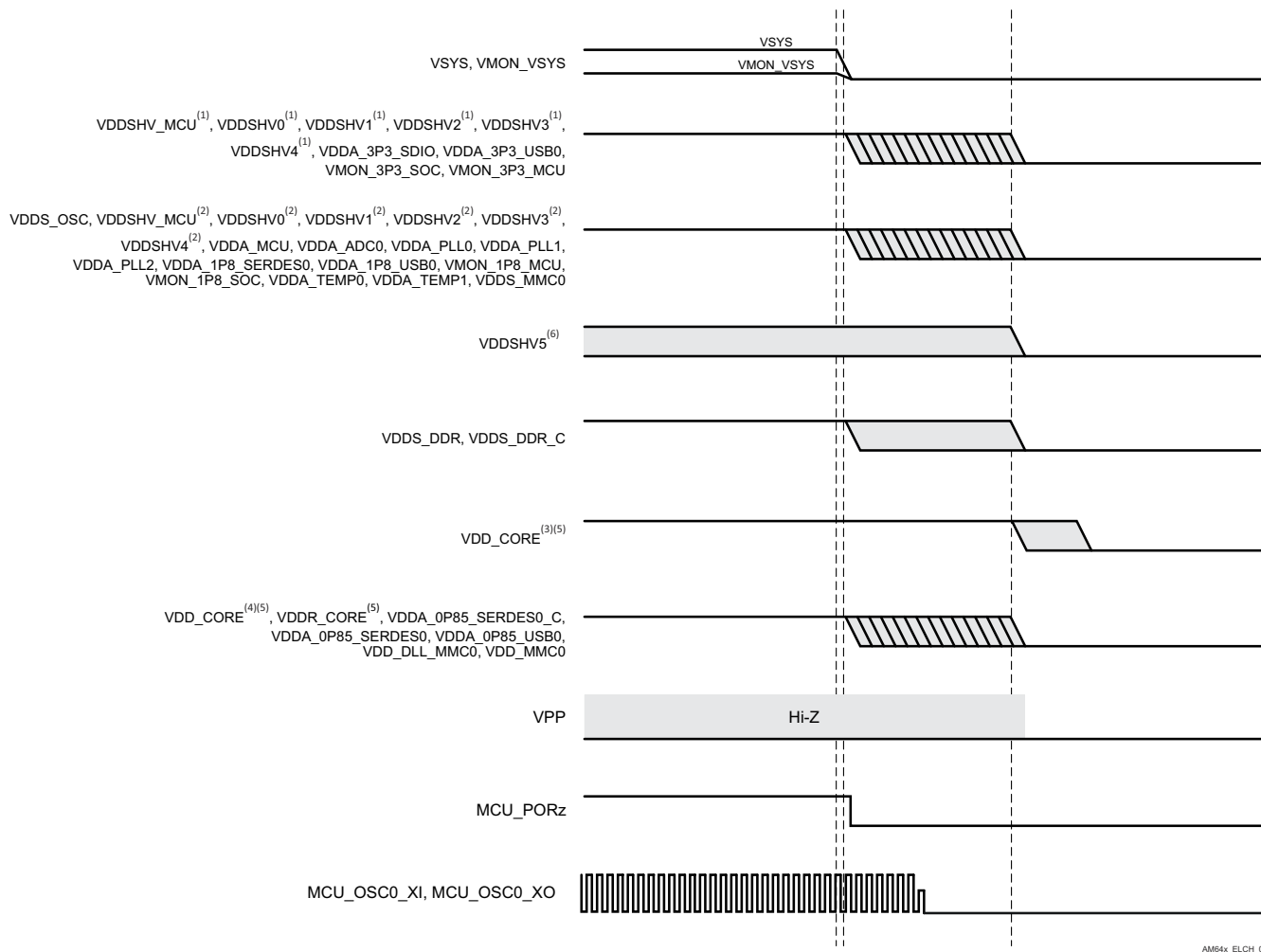
Figure 7-6. Power-Down Sequencing
