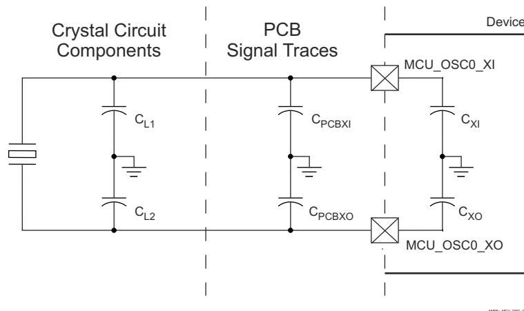
Figure 7-19. Load Capacitance
