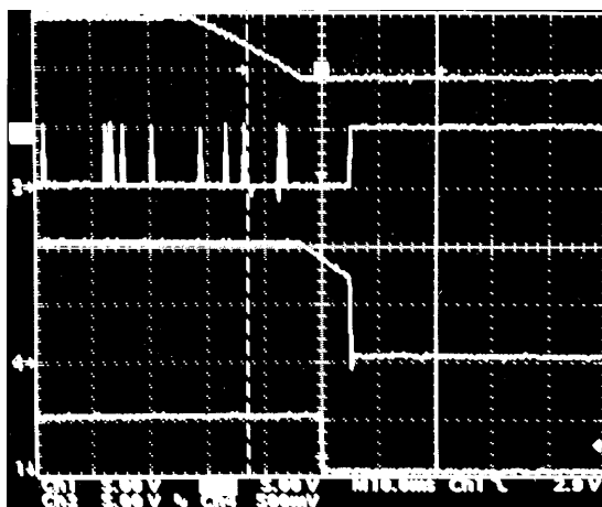
CH1: PGOOD, CH2: VIN, CH3: LDRV, CH4: V O Output 1V @ 0.02A, VIN = 9.75V, SKIP, L = 10μH, f = 300kHz, C OUT = 660μF
