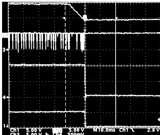
CH1: PGOOD, CH2: VIN, CH3: LDRV, CH4: V O Output 1V @ 0.02A, VIN = 9.75V, FPWM, L = 10μH, f = 300kHz, C OUT = 660μF
