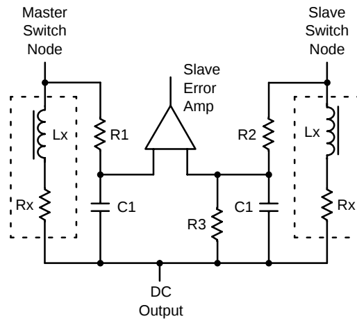
Figure 12. 40%/60% Current Sharing
