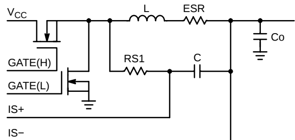
Figure 11. Inductor ESR Current Sensing
