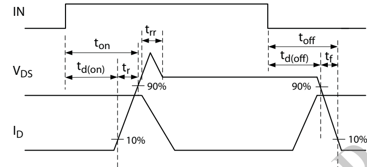
Switching Characteristics Definitions
