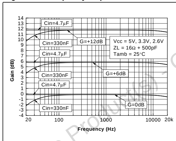
Figure 34. Frequency response
