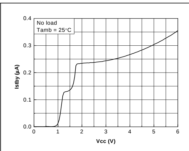
Figure 31. Standby current vs. supply voltage
