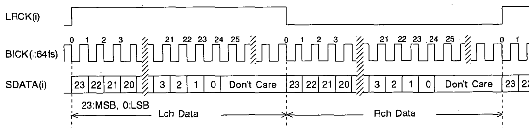
Figure 4 . Mode 2 Timing
