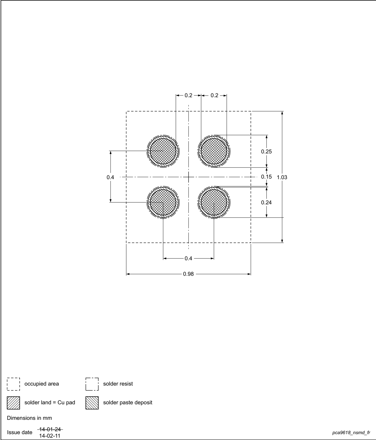
Fig 20. PCB footprint for PCA9618UK (WLCSP4); reflow soldering; Non-Solder Mask Defined (NSMD)
