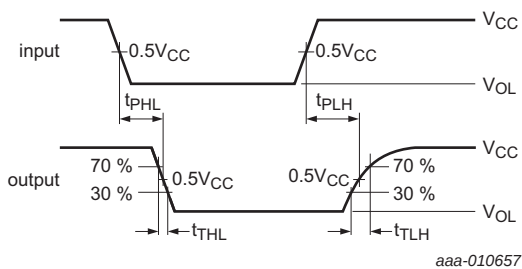
Fig 12. Propagation delay and transition times; port B to port A
