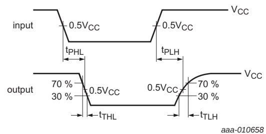
Fig 13. Propagation delay and transition times; port A to port B
