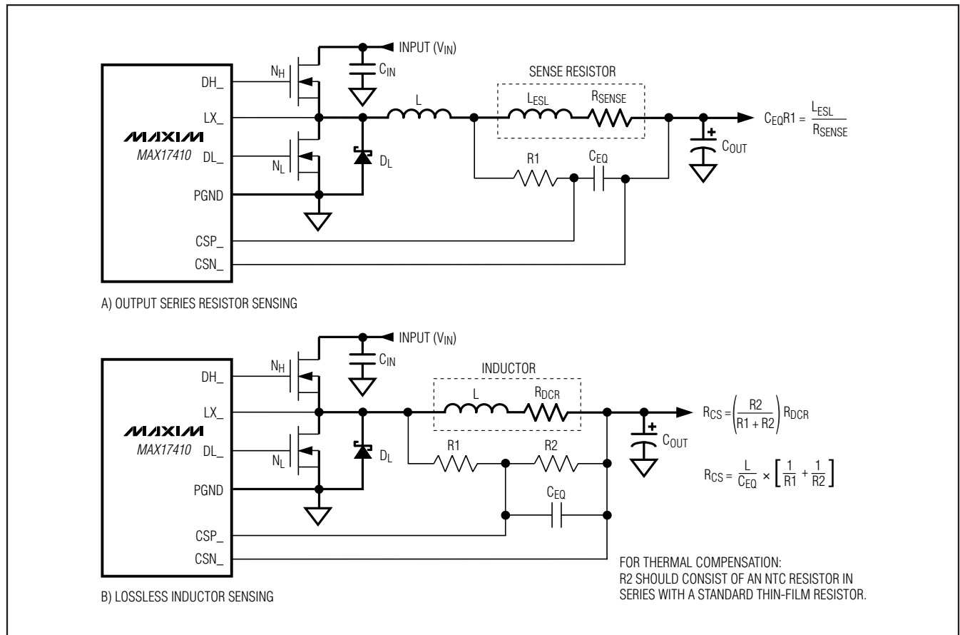
Figure 3. Current-Sense Methods
