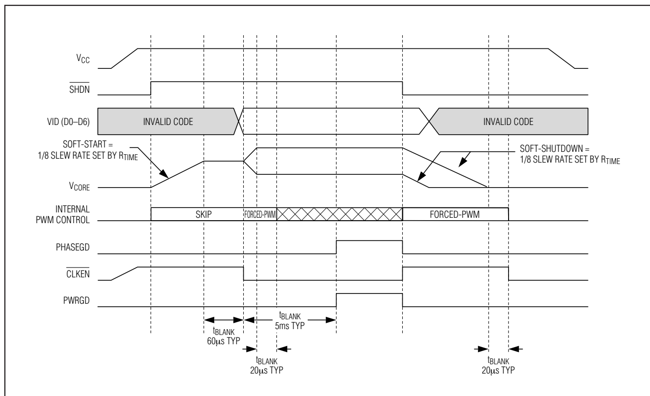
Figure 9. Power-Up and Shutdown Sequence Timing Diagram
