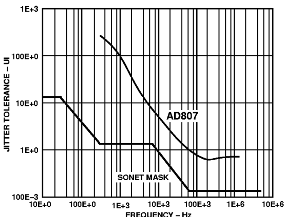
Figure 13. Jitter Tolerance
