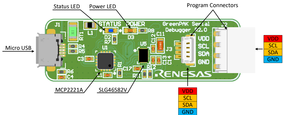
Figure 1: GreenPAK Serial Debugger Top View
