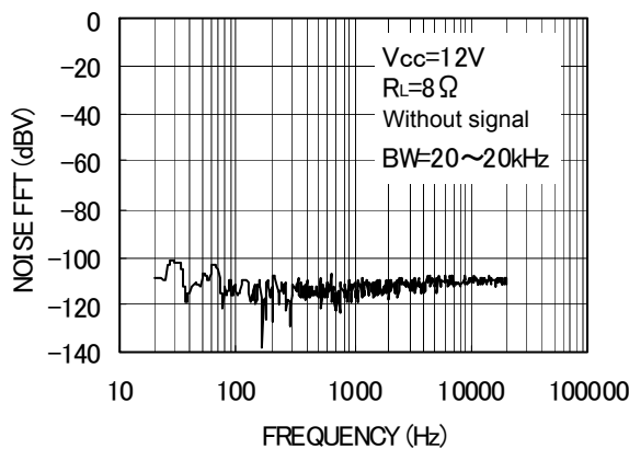
Fig. 12 FFT of Output Noise Voltage
