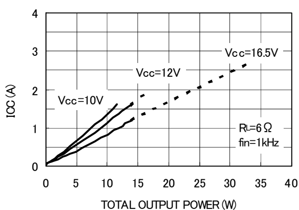
Fig. 21 Current consumption - Output power
