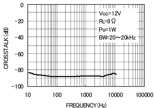
Fig. 4 Crosstalk - Frequency
