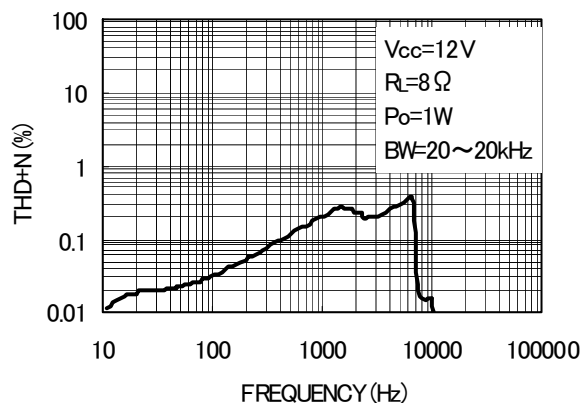
Fig. 2 THD+N — Frequency
