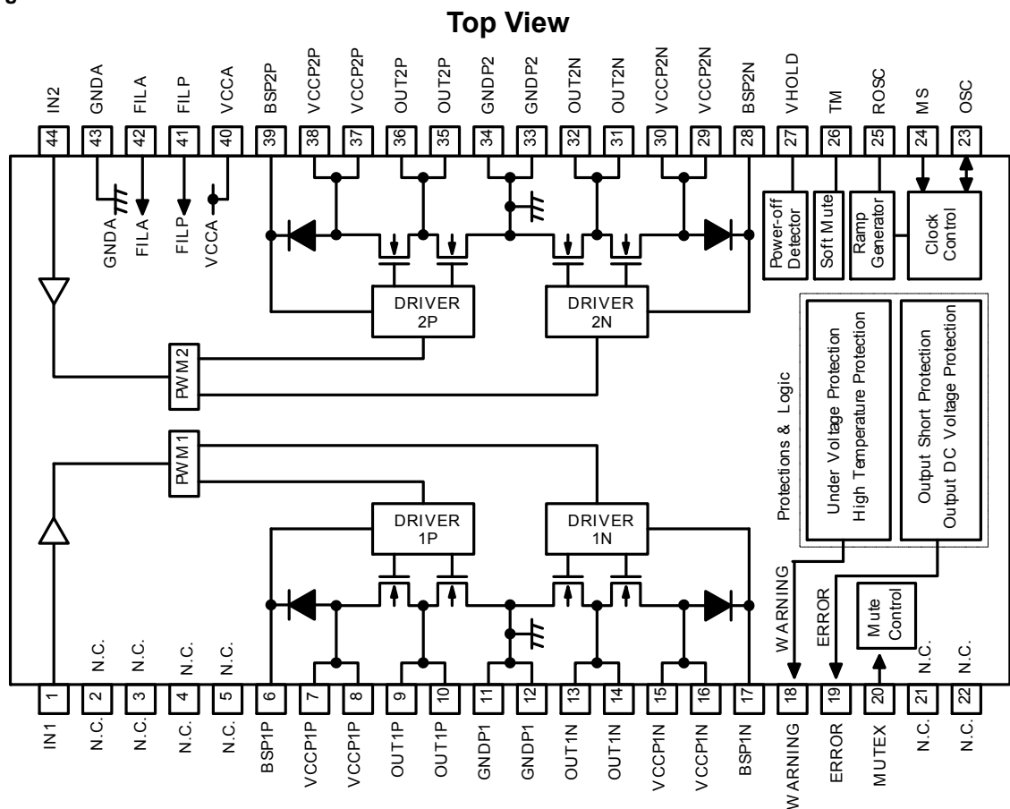
Fig. 22 Pin Assignment Diagram
