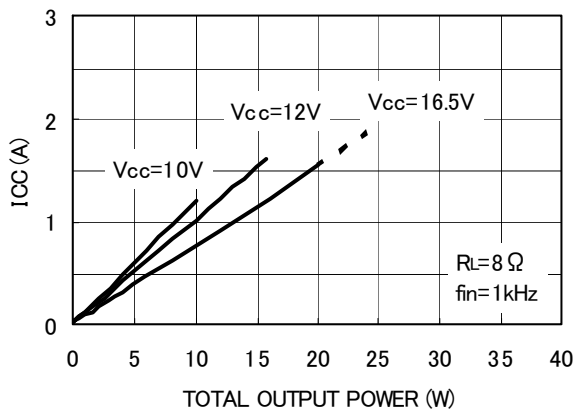
Fig. 10 Current consumption - Output power
