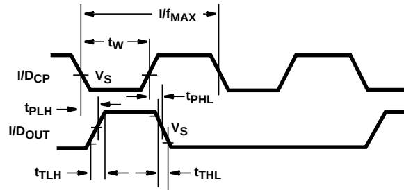
FIGURE 6. WAVEFORMS SHOWING THE CLOCK ( I/DCP ) TO OUTPUT ( I/DOU ) PROPAGATION DELAYS, CLOCK PULSE WIDTH, OUTPUT TRANSITION TIMES AND MAXIMUM CLOCK PULSE FREQUENCY
