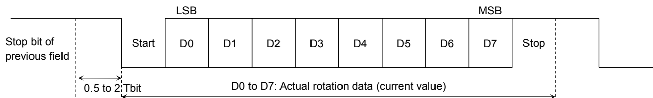
Figure 7.18 DATA1 Field
