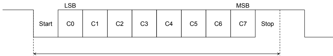
Figure 7.17 Checksum Field
