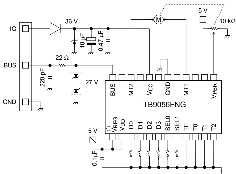
Figure 7.2 Example Slave Application Circuit
