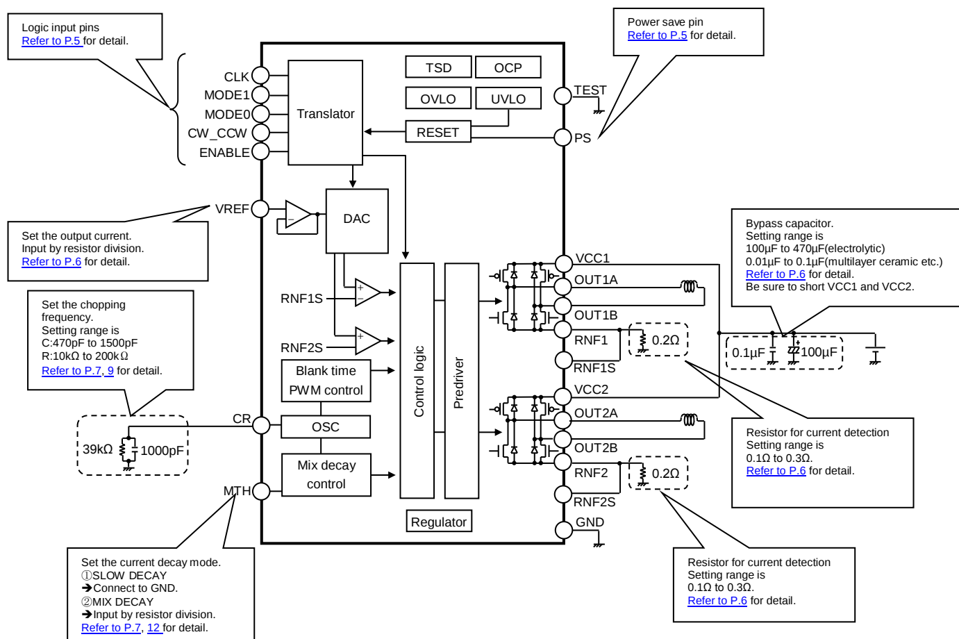
Figure 8. BD60223FP block diagram and applied circuit diagram
