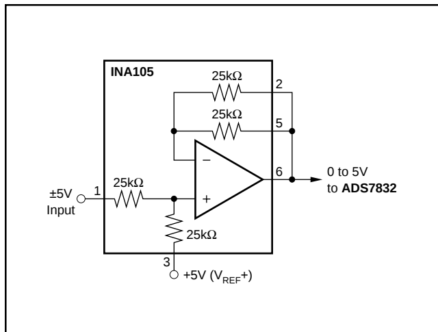
FIGURE 13. \pm 5\text{V} Input Range.
