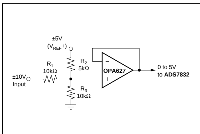
FIGURE 14. \pm 10\text{V} Input Range.
