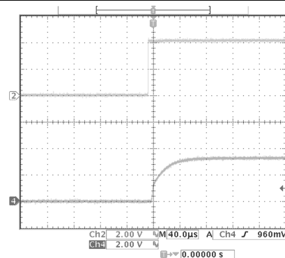
Figure 78. Enable Startup Time (LDO1)
