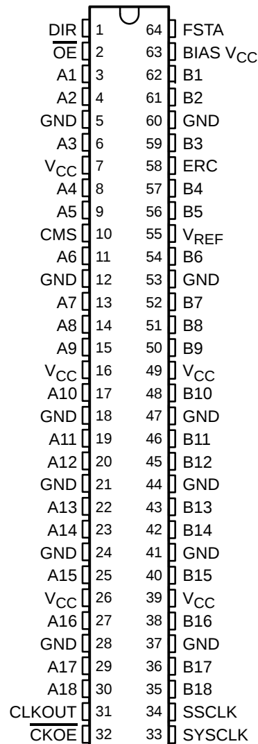
DGG PACKAGE (TOP VIEW)
