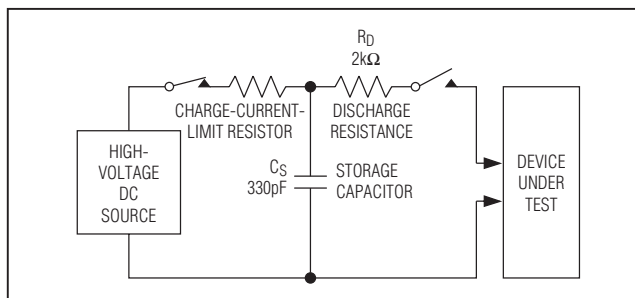
Figure 23. ISO 10605 Contact Discharge ESD Test Circuit
